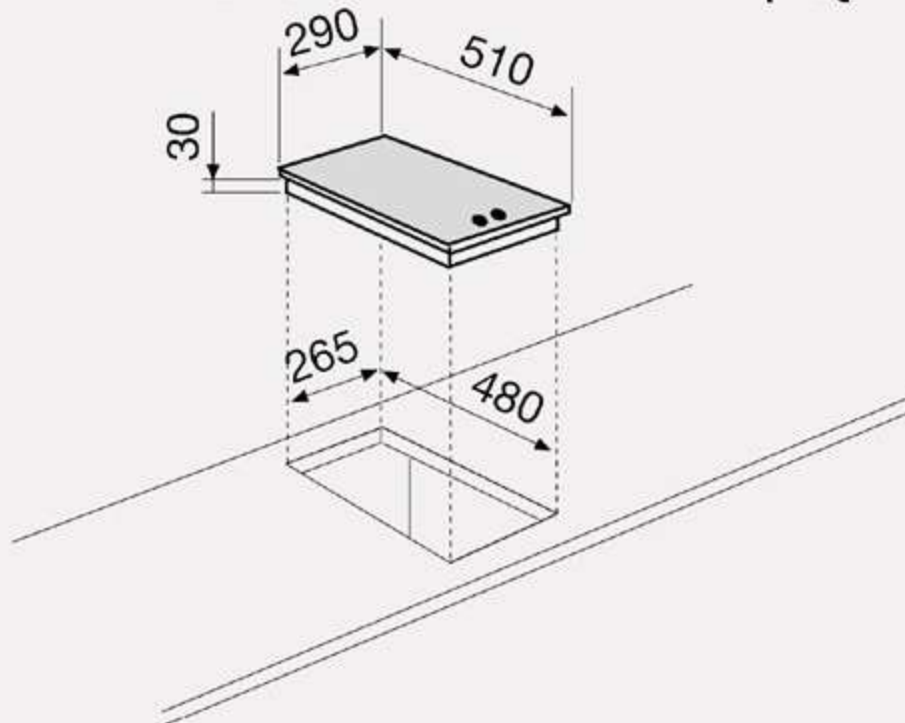
Product Dimensions (mm)
